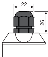
Variant "B" with cable outlet PG11
