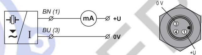
Connection diagram of the ULM level meter (variant -I) and inside view of the connector
